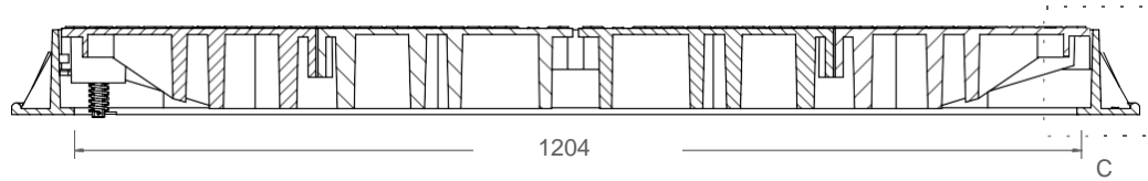
Section B-B
