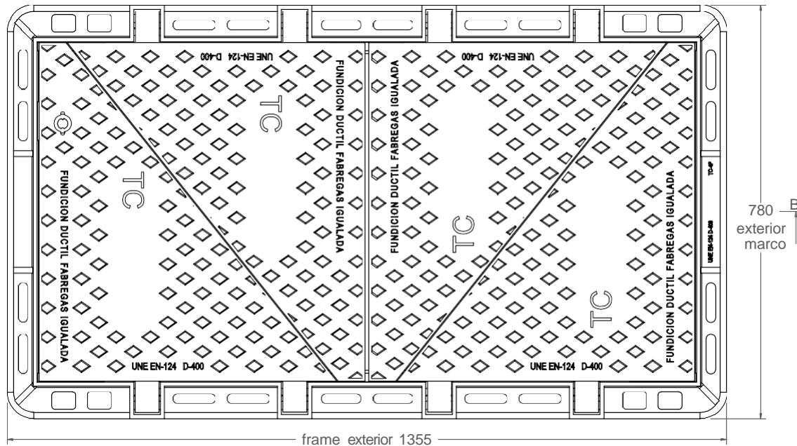
frame exterior 1355 upside view 1:10
